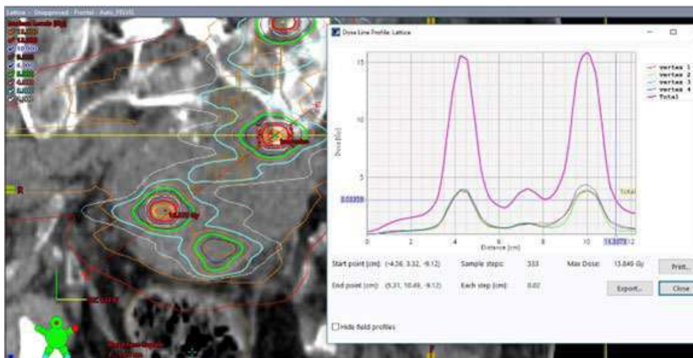
Figure 2. Dose profiles showing the achieved valleys and peaks
