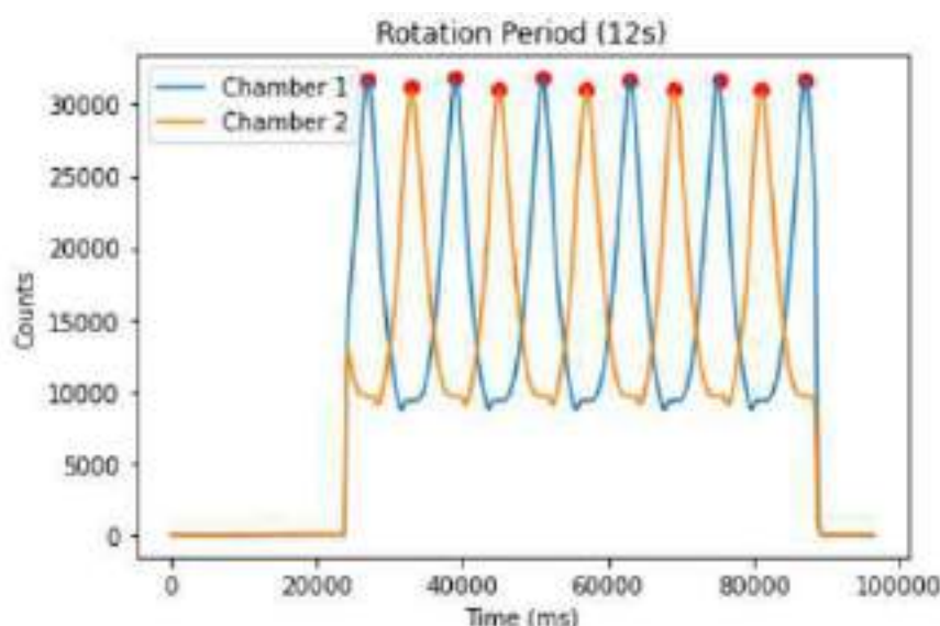
Figure 2. Measurements from chamber 1 (blue) and chamber 2 (orange) for a rotation period of 12s. The red circles represent the position of the peaks detected automatically by the program.
